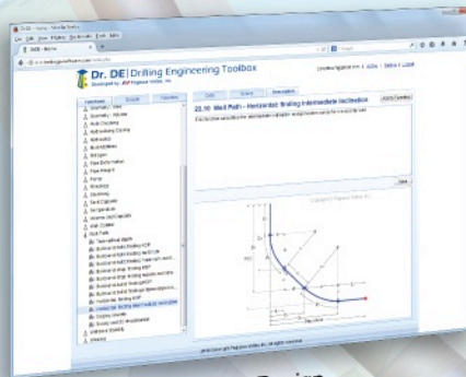
Well Path Design
