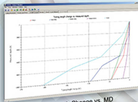
Tubing Length Change vs. MD
