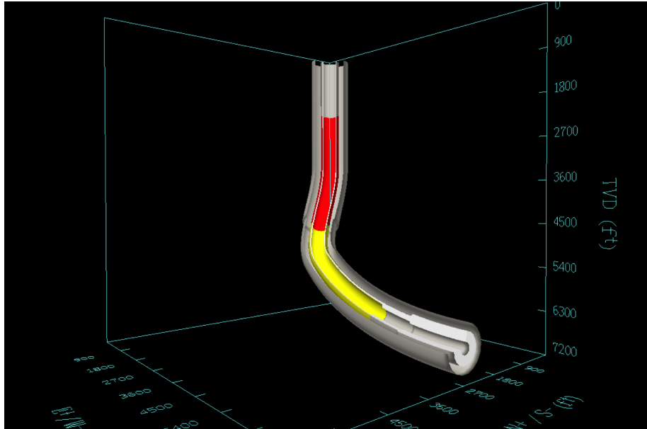
Figure 4: 3D Video Screenshot of Buckling in a String
