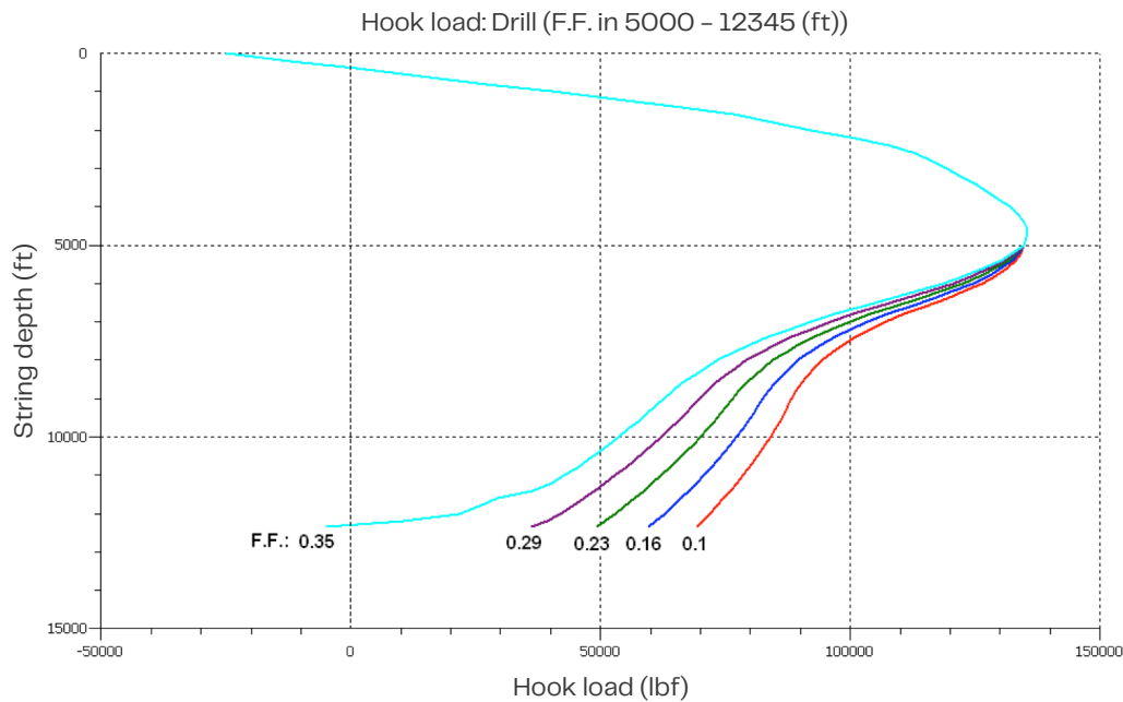
Figure 3: Friction Factor Sensitivity Graph
